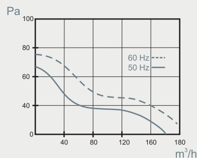
Performance curves
